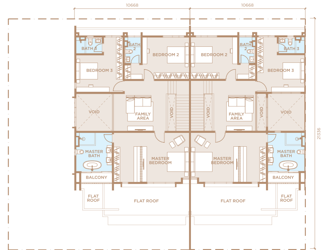
FIRST FLOOR
